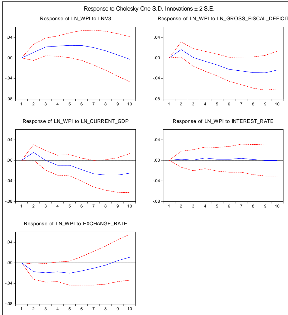
Figure 1: Impulse Response of WPI to Other Variables
